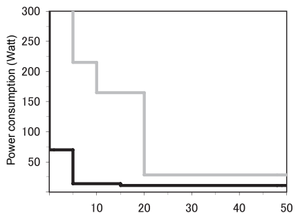
Power consumption and default times of MFC-9120CN during time elapsed after the last print
