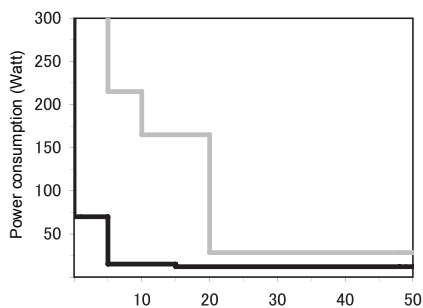
Power consumption and default times of MFC-9320CW during time elapsed after the last print
